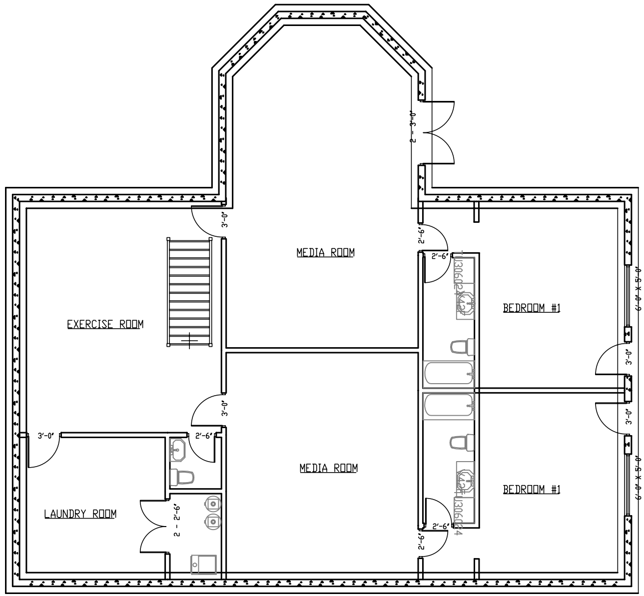
BASEMENT LAYOUT
